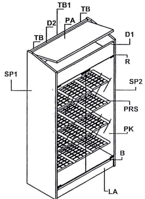
FINAL ASSEMBLING
